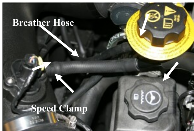
17. Install the 1/2"x 6" breather hose between the nipple on the air intake tube and the hard plastic crankcase breather tube. Refer to step #2. Install one #16 speed clamp (#20) over the breather hose at the nipple as shown.
